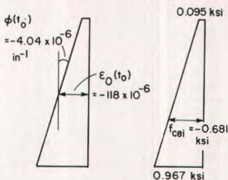
(b) STRAIN AND STRESS AT t_i , IMMEDIATELY AFTER PRESTRESSING
